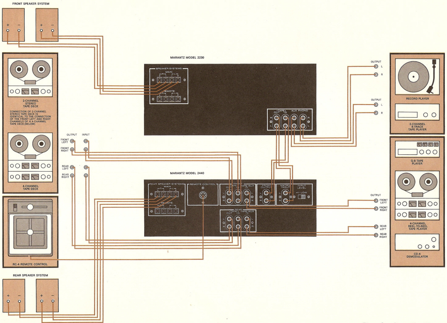
Figure 8. Connection Diagram
