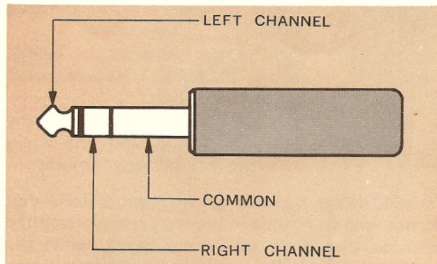
Figure 6. Stereophone Plug
